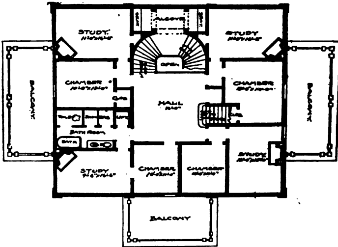
SECOND FLOOR PLAN, ZETA CHAPTER HOUSE
